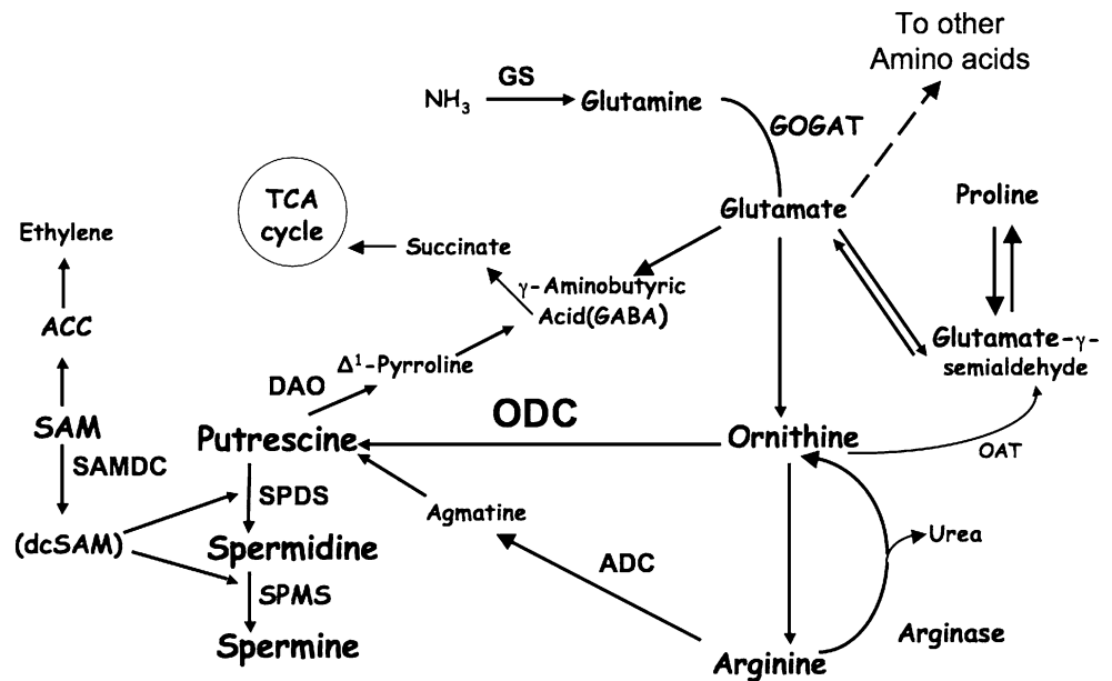
Fig. 1 Biosynthesis pathways showing interconnections between biogenic amines, amino acids, TCA cycle and ethylene
